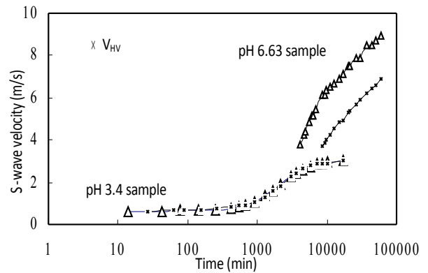
Fig. 1 Evolution of the shear wave velocity for the two clay samples.
